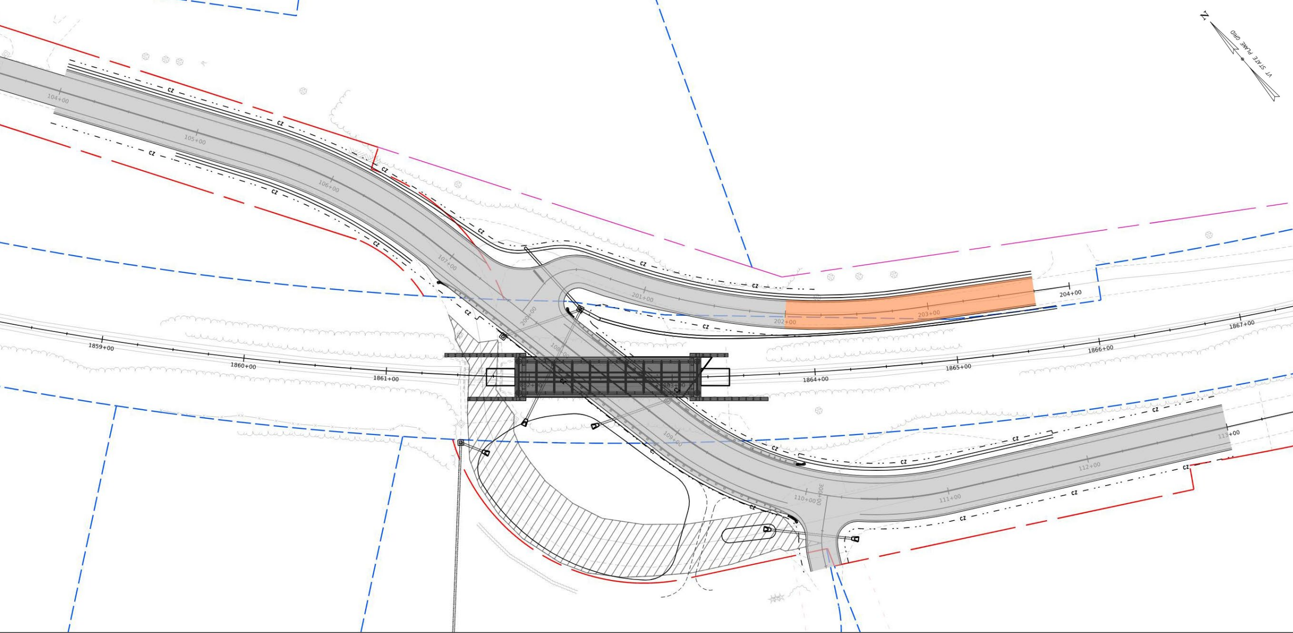
Proposed Configuration Plan
