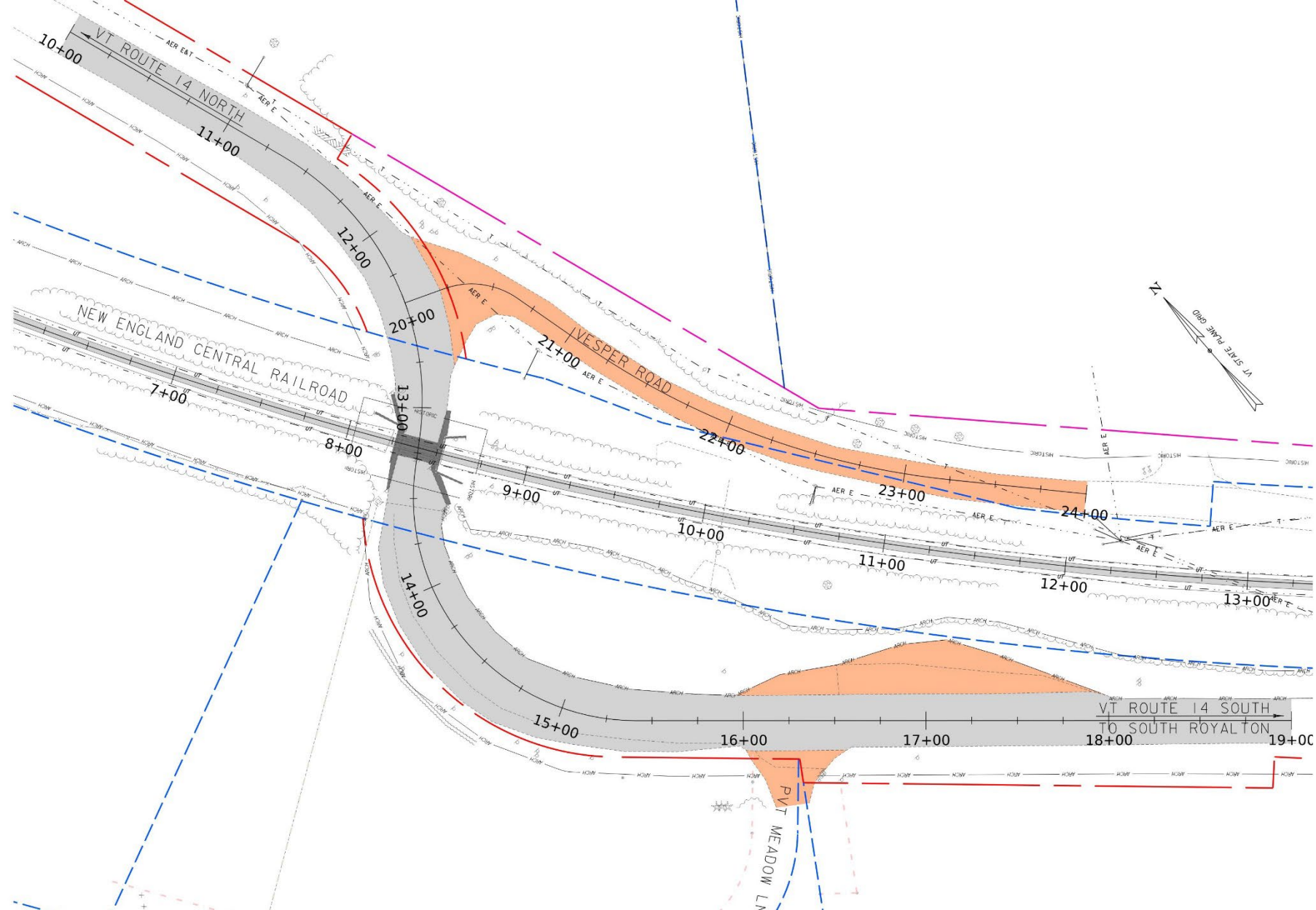
Existing Conditions Plan
